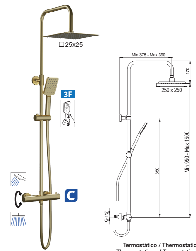
Termostático / Thermostatic Thermostatique / Termostatico 20NITC25NID09 320,20€ 6024X2 9 l/min 3 bar +4,80€
